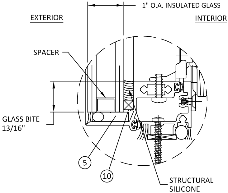
GLAZING DETAIL 1
