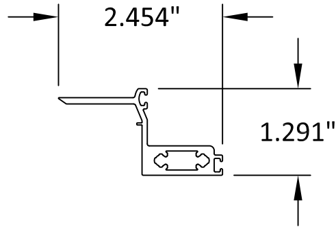
3 VENT RAIL / STILE 6063-T5
