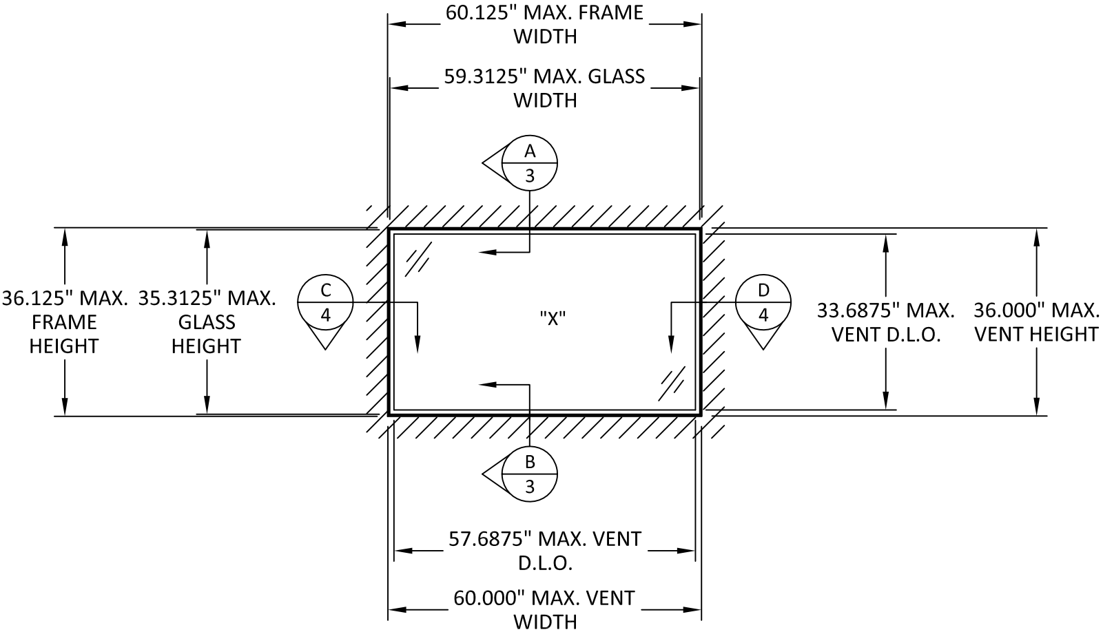
TYPICAL ELEVATION
