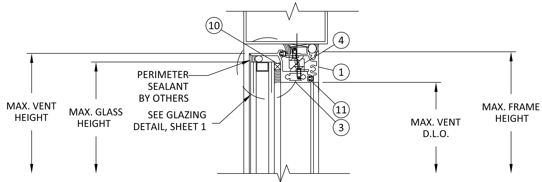
A 3 VERTICAL SECTION THROUGH FRAME INSTALLATION
