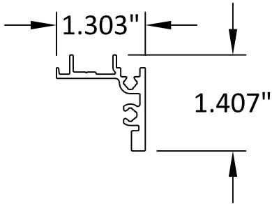
1 FRAME HEAD AND SILL 6063-T5
