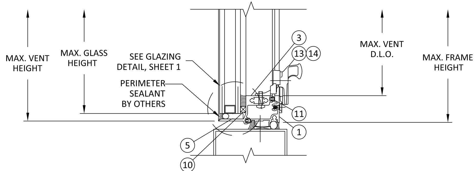
B 3 VERTICAL SECTION THROUGH FRAME INSTALLATION
