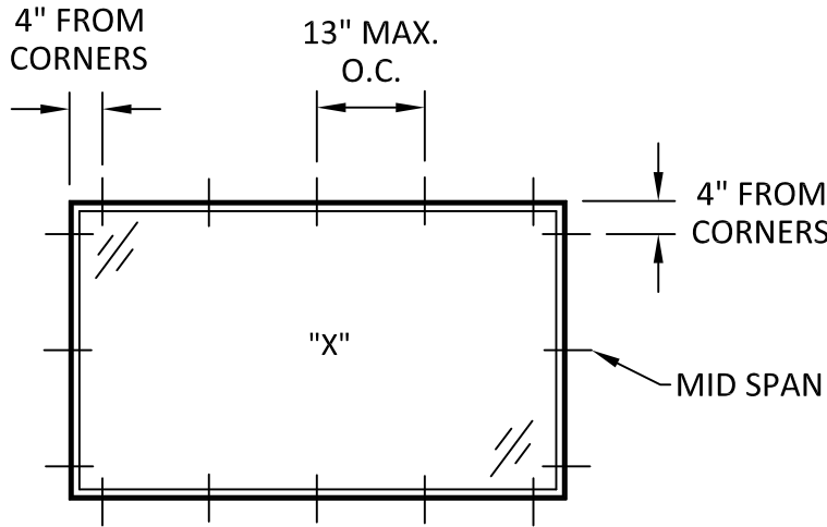
ANCHOR LAYOUT TYPICAL FOR THROUGH FRAME INSTALLATION
